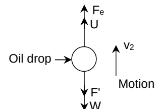
Fig. Upward motion of oil drop under electric field
